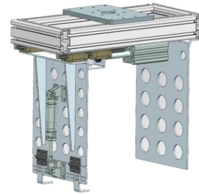
Double-acting gripper
