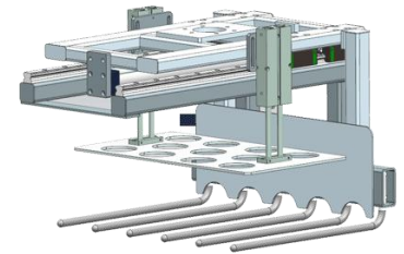
Drawer-type gripper
