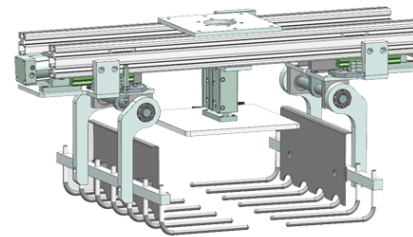
Clamping gripper
